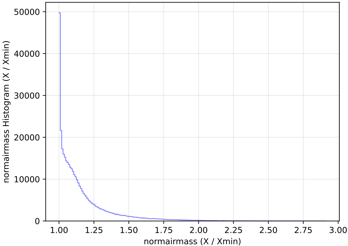
too_elab_r64_d3_ugrizy_v3.4_10yrs All sky y band: normairmass Histogram
