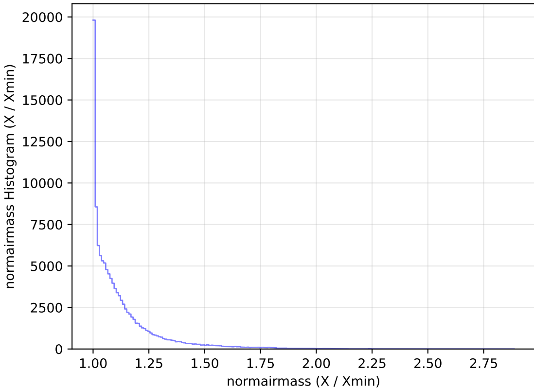
too_elab_r64_d3_ugrizy_v3.4_10yrs All sky u band: normairmass Histogram
