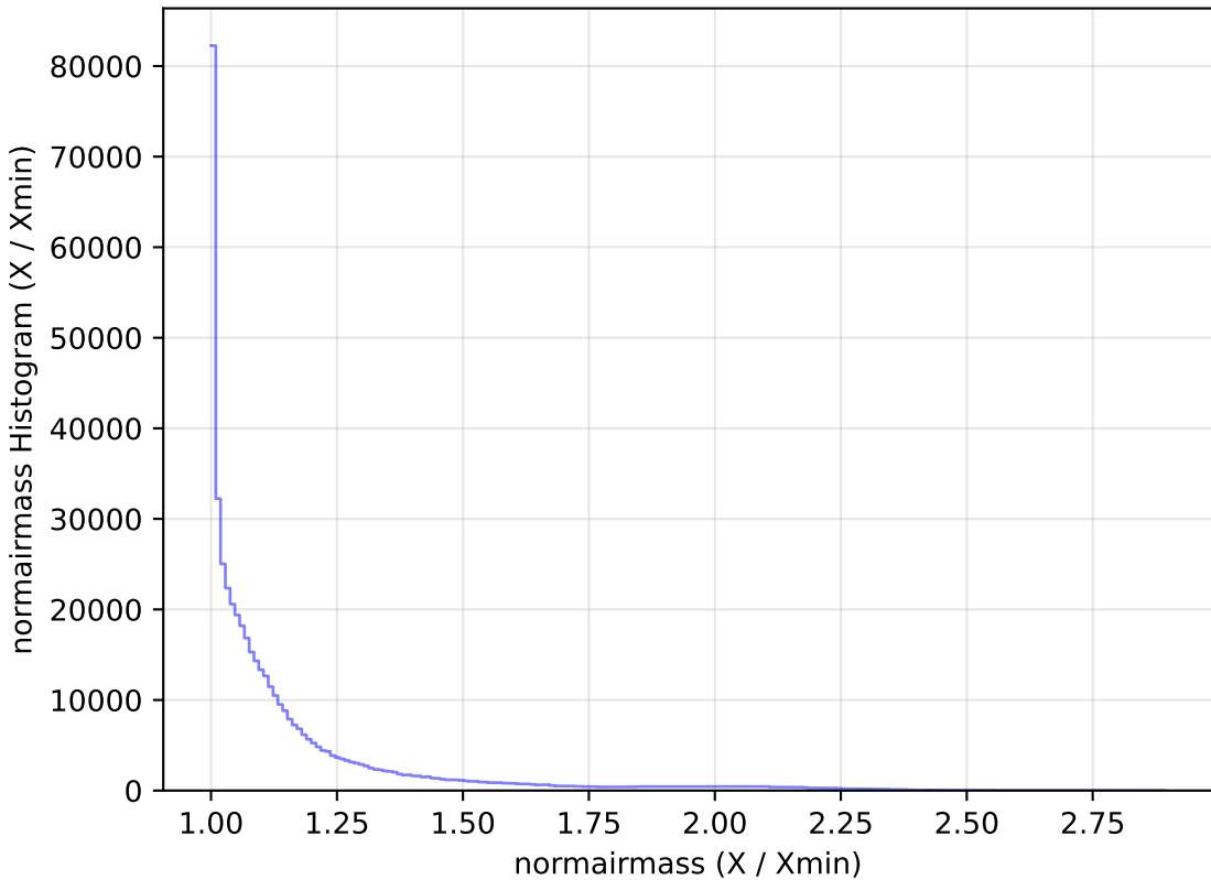
too_elab_r64_d3_ugrizy_v3.4_10yrs All sky r band: normairmass Histogram
