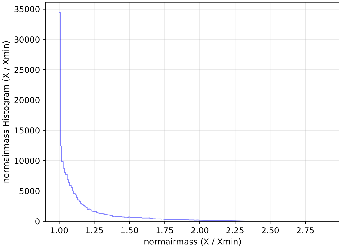
too_elab_r64_d3_ugrizy_v3.4_10yrs All sky g band: normairmass Histogram
