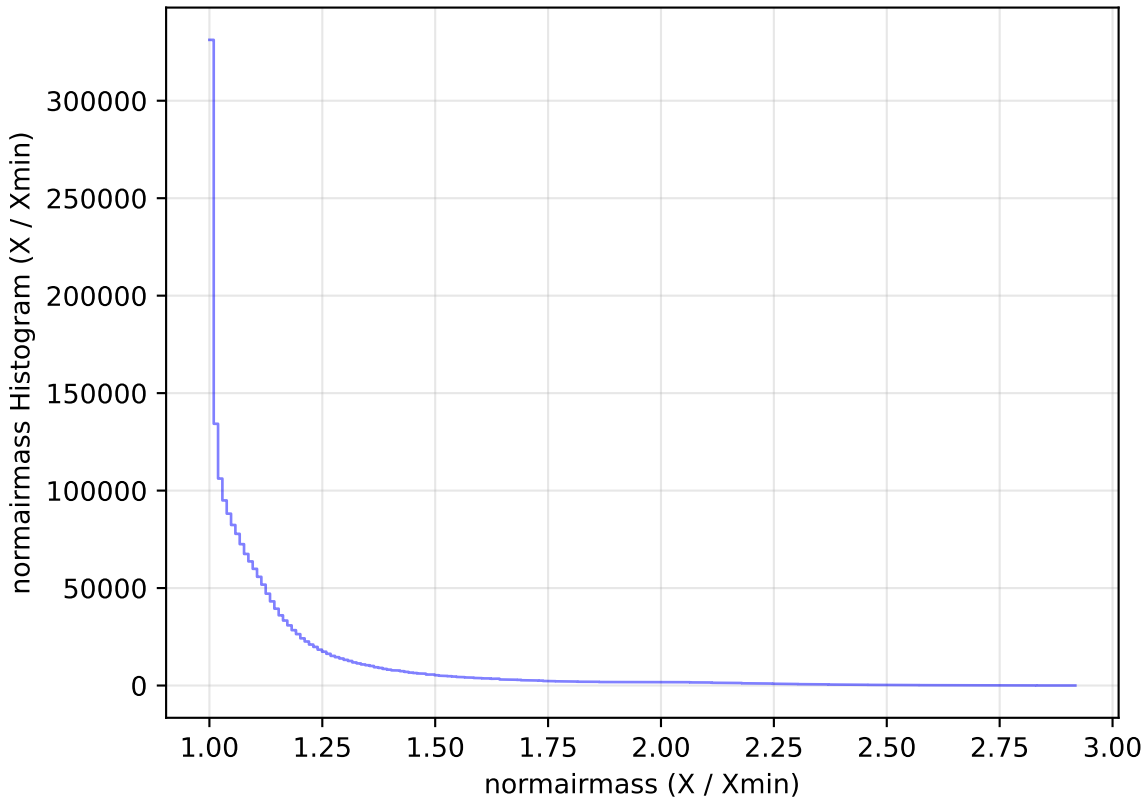
too_elab_r64_d3_ugrizy_v3.4_10yrs All sky all bands: normairmass Histogram
