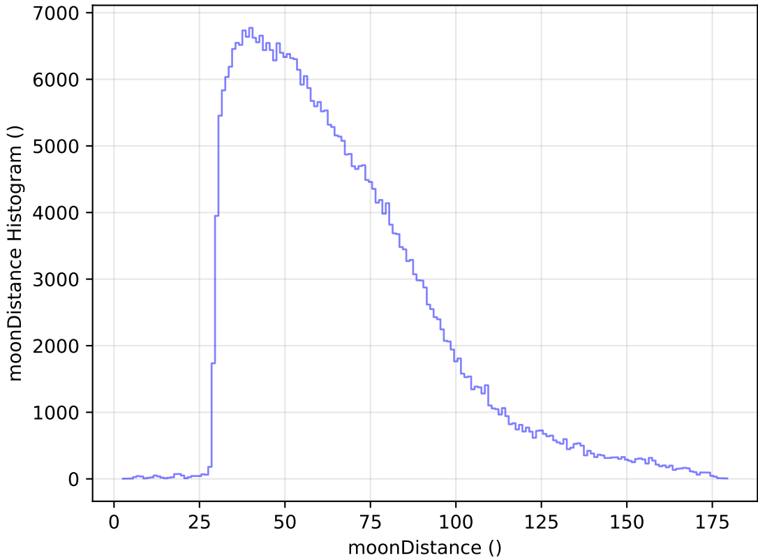
too_elab_r64_d3_ugrizy_v3.4_10yrs WFD y band: moonDistance Histogram
