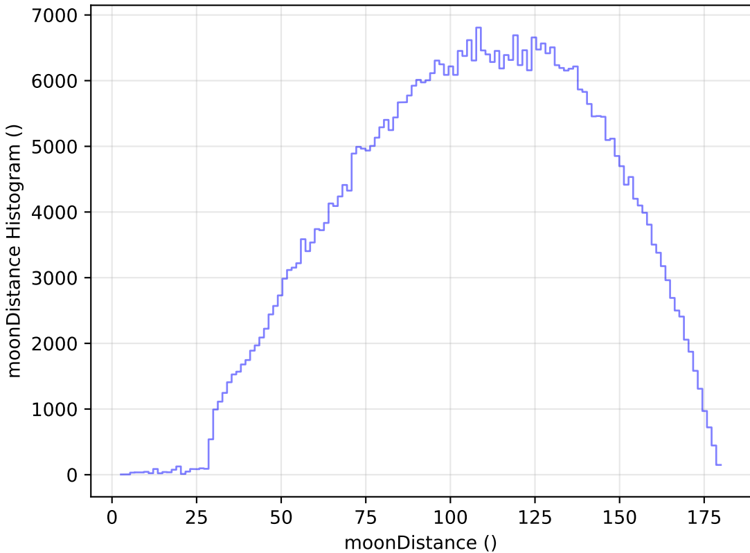
too_elab_r64_d3_ugrizy_v3.4_10yrs WFD r band: moonDistance Histogram
