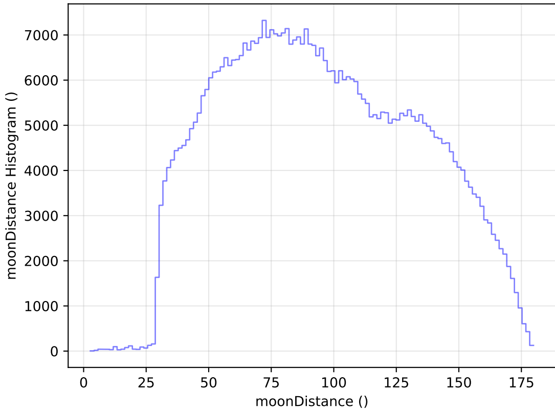
too_elab_r64_d3_ugrizy_v3.4_10yrs WFD i band: moonDistance Histogram
