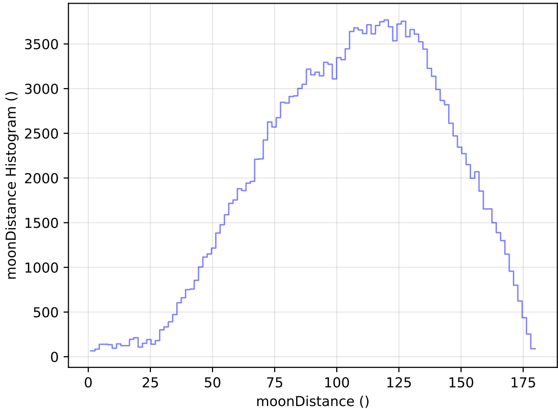
too_elab_r64_d3_ugrizy_v3.4_10yrs WFD g band: moonDistance Histogram
