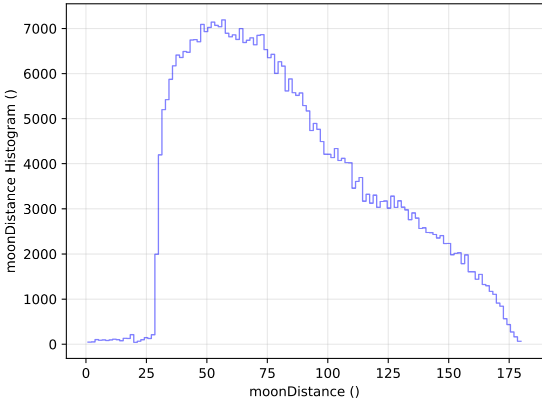
too_elab_r64_d3_ugrizy_v3.4_10yrs All sky z band: moonDistance Histogram
