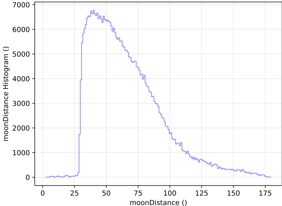
too_elab_r64_d3_ugrizy_v3.4_10yrs All sky y band: moonDistance Histogram
