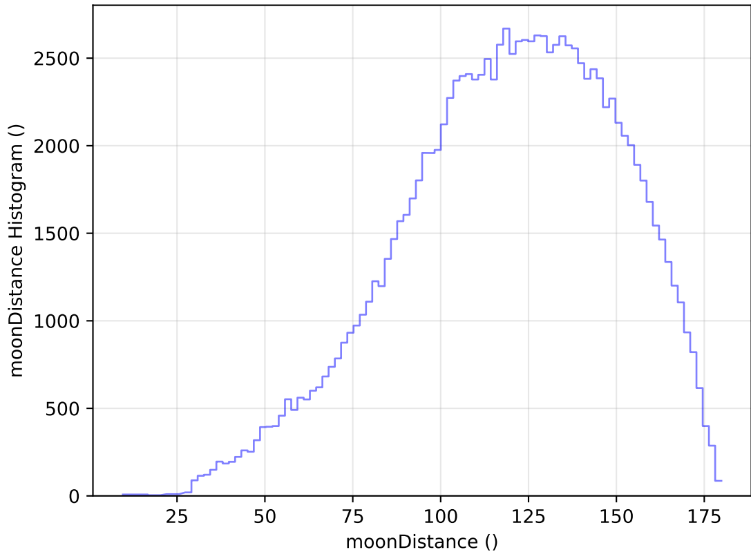
too_elab_r64_d3_ugrizy_v3.4_10yrs All sky u band: moonDistance Histogram
