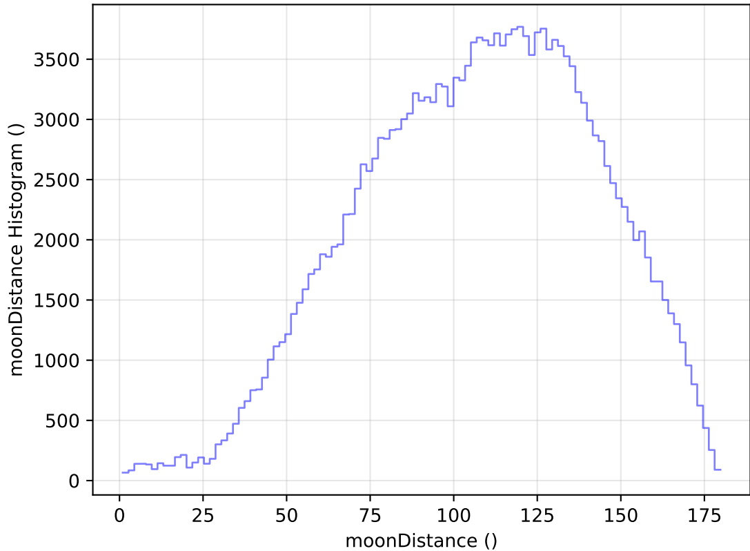
too_elab_r64_d3_ugrizy_v3.4_10yrs All sky g band: moonDistance Histogram
