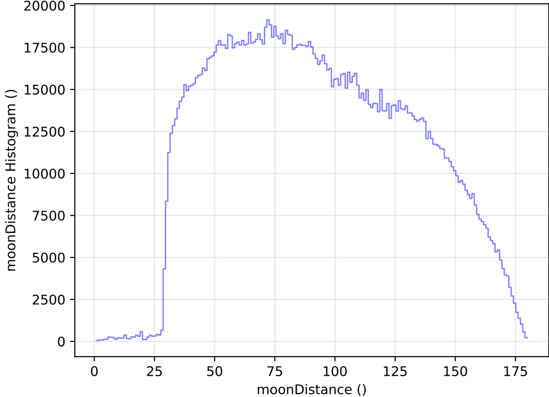
too_elab_r64_d3_ugrizy_v3.4_10yrs All sky all bands: moonDistance Histogram
