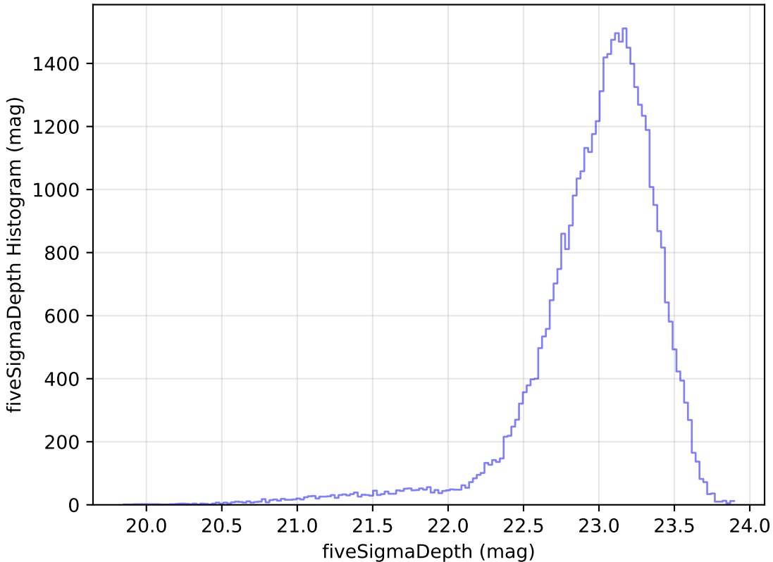
too_elab_r64_d3_ugrizy_v3.4_10yrs Yr 1 z band: fiveSigmaDepth Histogram
