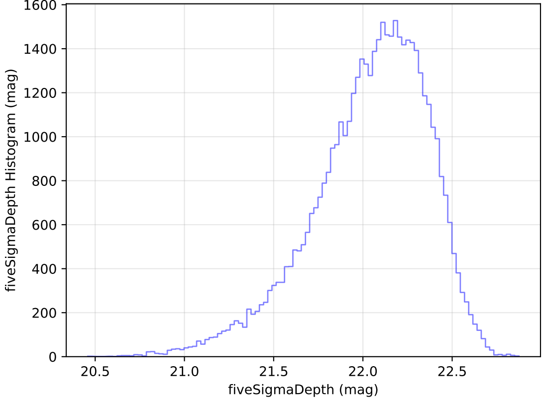
too_elab_r64_d3_ugrizy_v3.4_10yrs Yr 1 y band: fiveSigmaDepth Histogram
