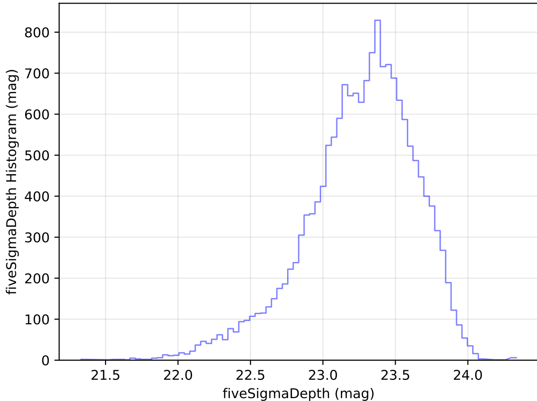
too_elab_r64_d3_ugrizy_v3.4_10yrs Yr 1 u band: fiveSigmaDepth Histogram
