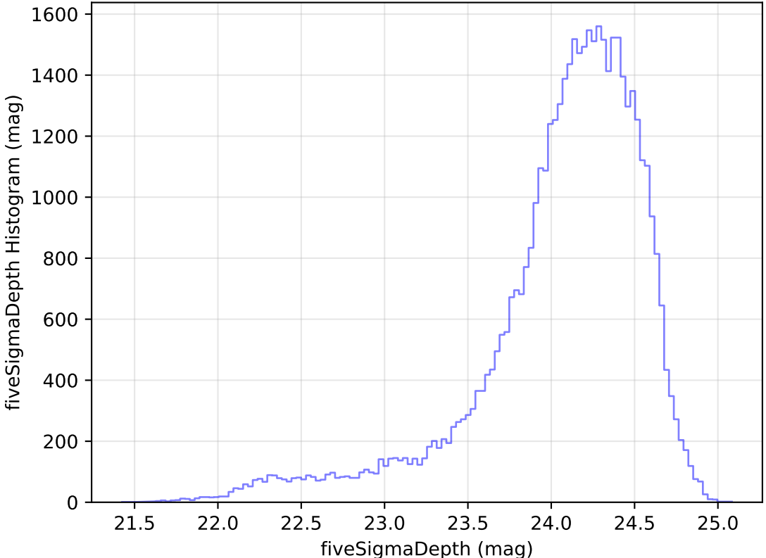
too_elab_r64_d3_ugrizy_v3.4_10yrs Yr 1 r band: fiveSigmaDepth Histogram
