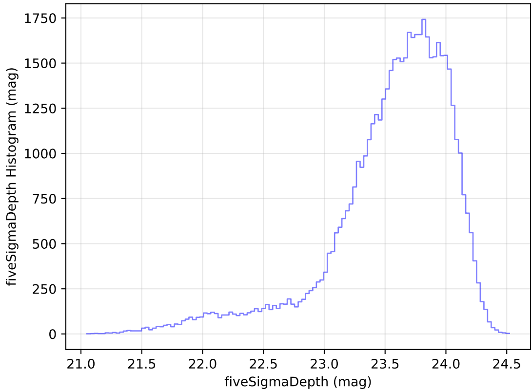
too_elab_r64_d3_ugrizy_v3.4_10yrs Yr 1 i band: fiveSigmaDepth Histogram
