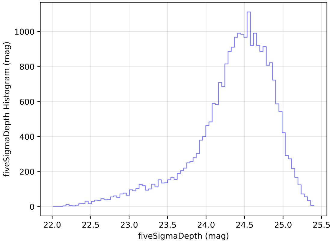
too_elab_r64_d3_ugrizy_v3.4_10yrs Yr 1 g band: fiveSigmaDepth Histogram
