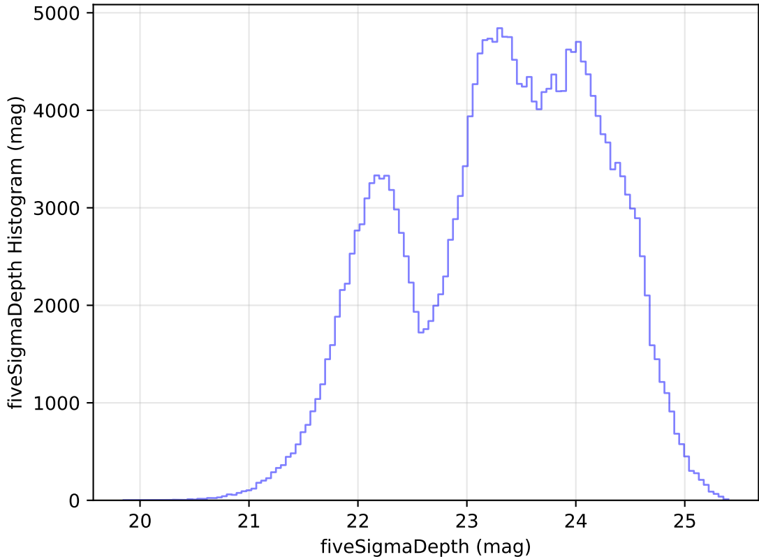
too_elab_r64_d3_ugrizy_v3.4_10yrs Yr 1 all bands: fiveSigmaDepth Histogram
