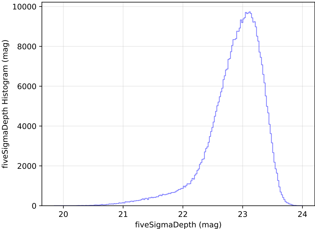
too_elab_r64_d3_ugrizy_v3.4_10yrs WFD z band: fiveSigmaDepth Histogram
