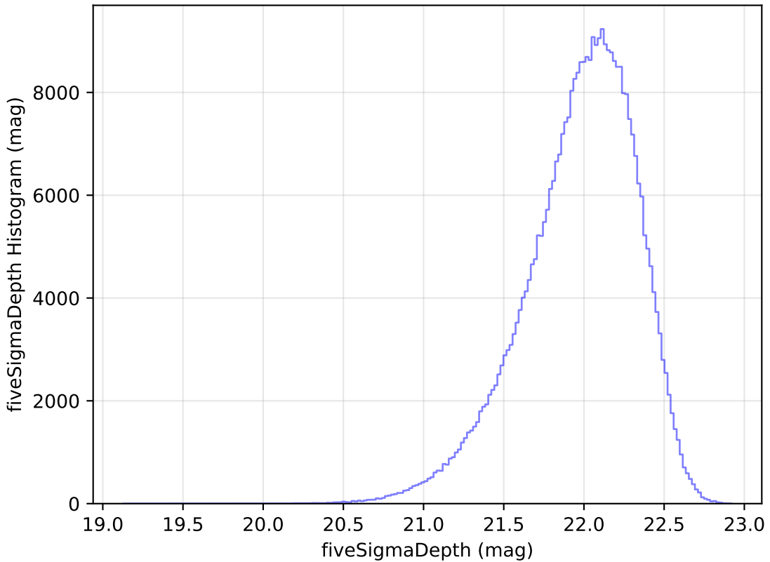
too_elab_r64_d3_ugrizy_v3.4_10yrs WFD y band: fiveSigmaDepth Histogram
