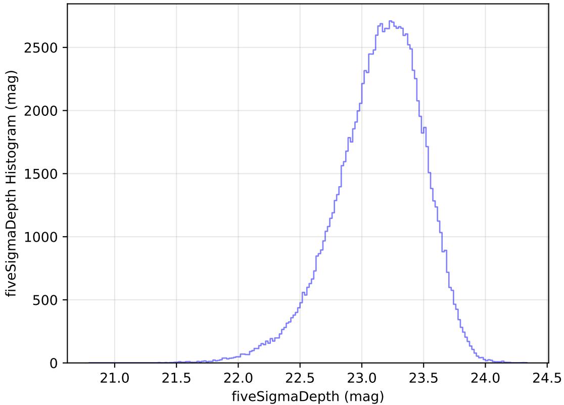
too_elab_r64_d3_ugrizy_v3.4_10yrs WFD u band: fiveSigmaDepth Histogram
