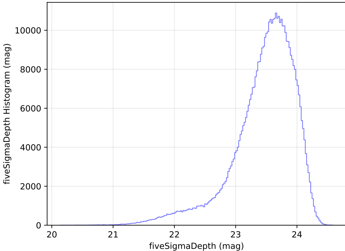
too_elab_r64_d3_ugrizy_v3.4_10yrs_WFD_i_band: fiveSigmaDepth Histogram
