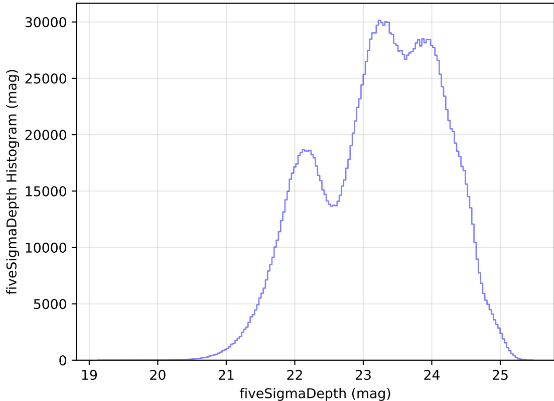
too_elab_r64_d3_ugrizy_v3.4_10yrs WFD all bands: fiveSigmaDepth Histogram
