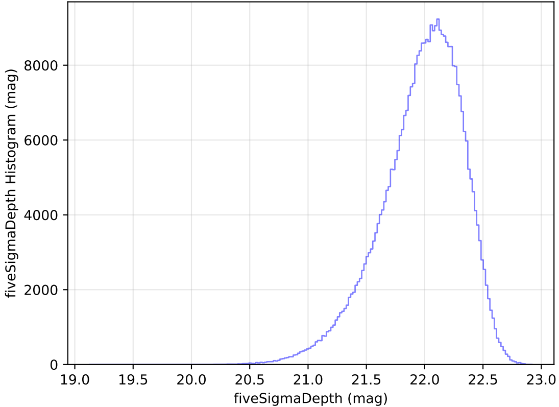
too_elab_r64_d3_ugrizy_v3.4_10yrs All sky y band: fiveSigmaDepth Histogram
