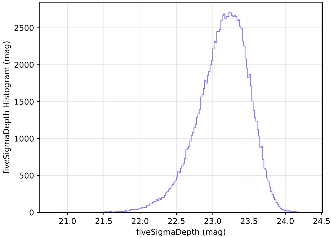
too_elab_r64_d3_ugrizy_v3.4_10yrs All sky u band: fiveSigmaDepth Histogram
