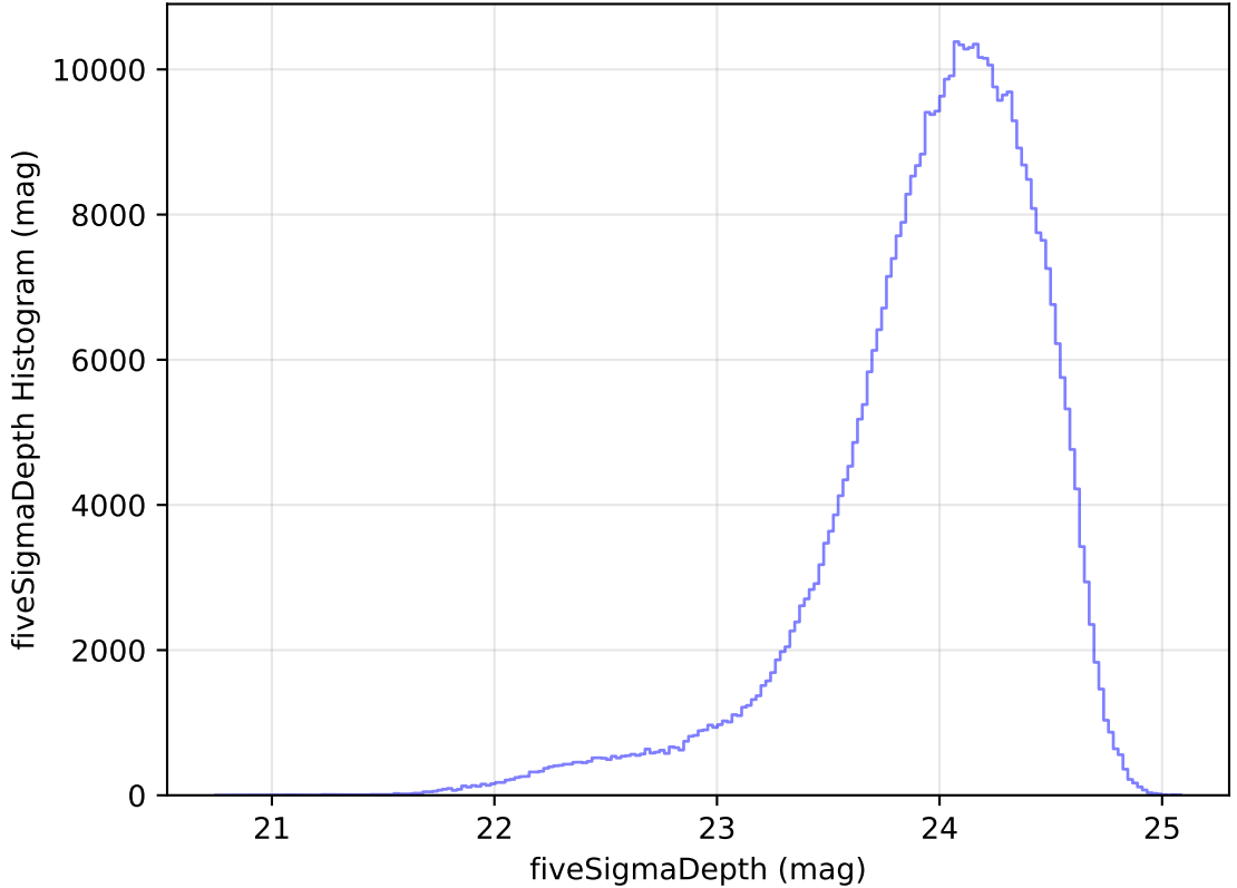
too_elab_r64_d3_ugrizy_v3.4_10yrs All sky r band: fiveSigmaDepth Histogram
