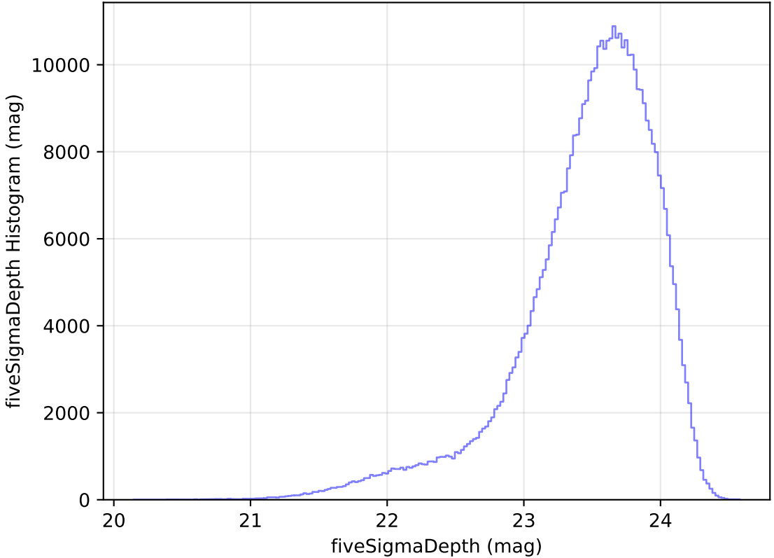
too_elab_r64_d3_ugrizy_v3.4_10yrs All sky i band: fiveSigmaDepth Histogram
