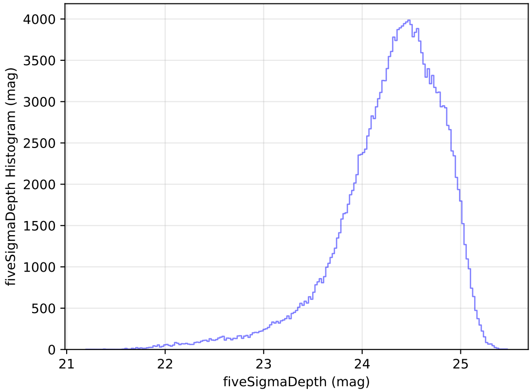
too_elab_r64_d3_ugrizy_v3.4_10yrs All sky g band: fiveSigmaDepth Histogram
