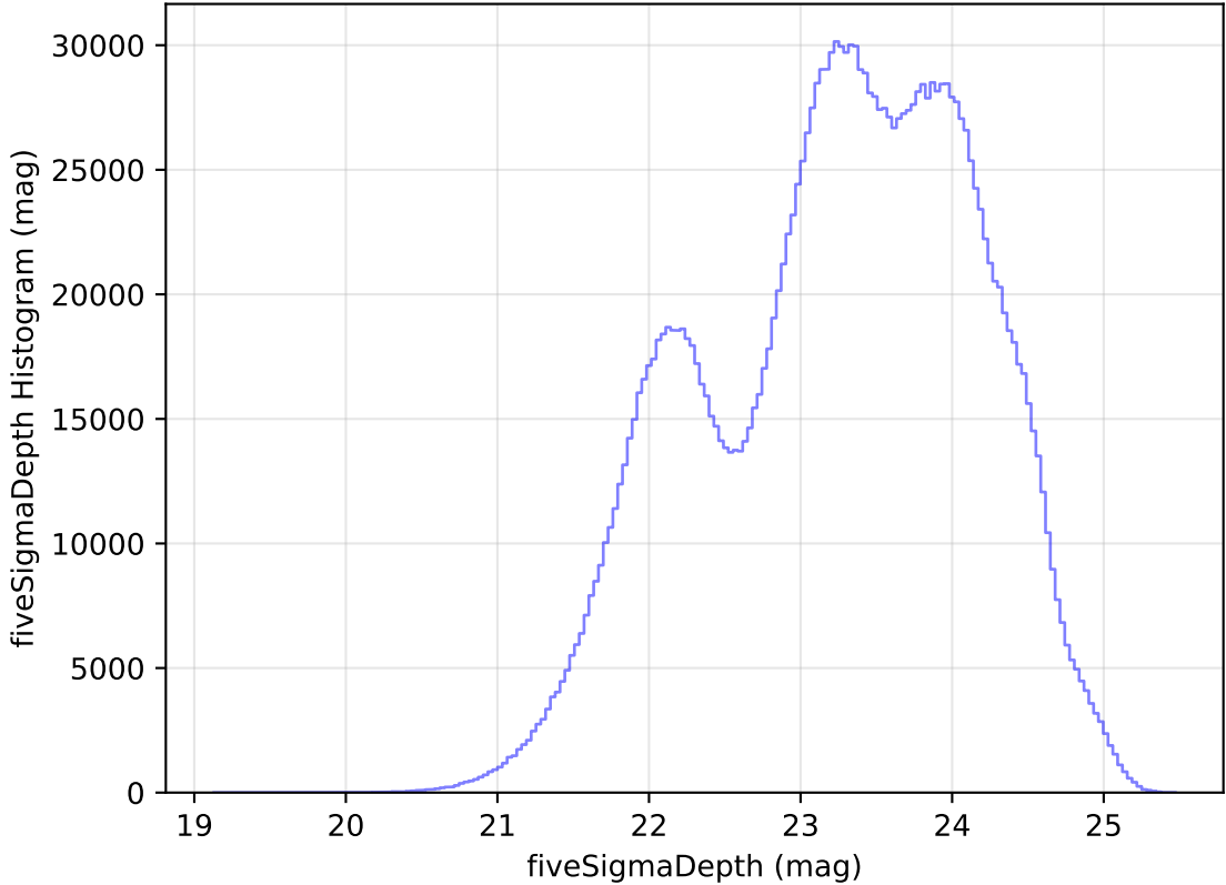
too_elab_r64_d3_ugrizy_v3.4_10yrs All sky all bands: fiveSigmaDepth Histogram
