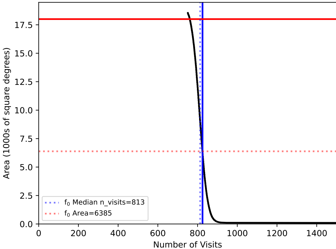
too_elab_r64_d3_ugrizy_v3.4_10yrs WFD: f0
