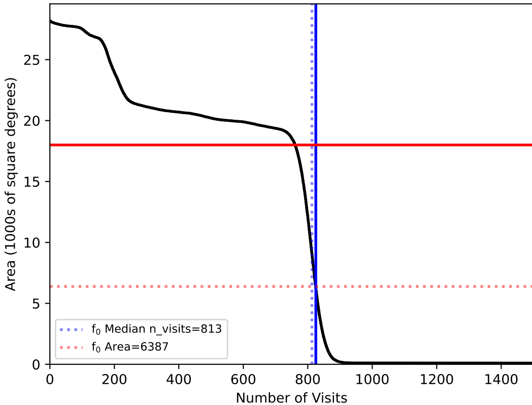
too_elab_r64_d3_ugrizy_v3.4_10yrs All sky: f0
