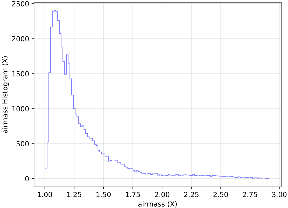
too_elab_r64_d3_ugrizy_v3.4_10yrs Yr 1 z band: airmass Histogram
