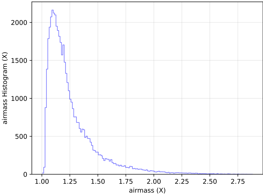
too_elab_r64_d3_ugrizy_v3.4_10yrs Yr 1 y band: airmass Histogram
