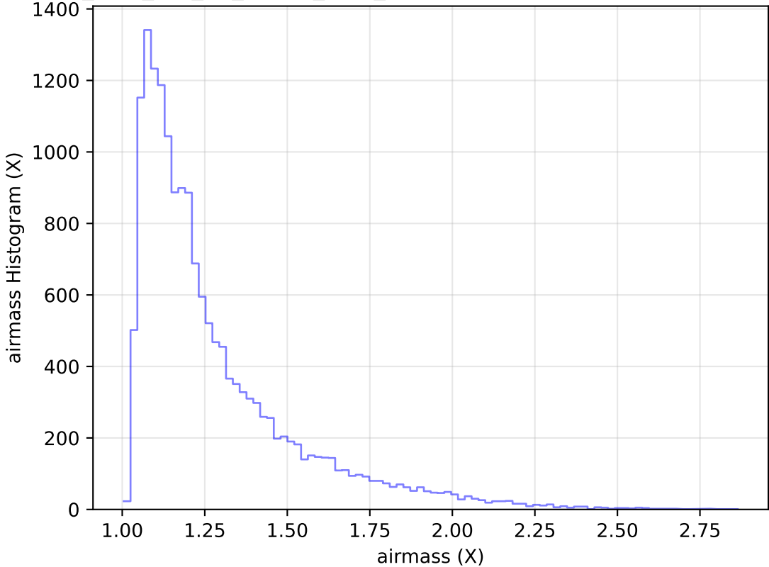
too_elab_r64_d3_ugrizy_v3.4_10yrs Yr 1 u band: airmass Histogram
