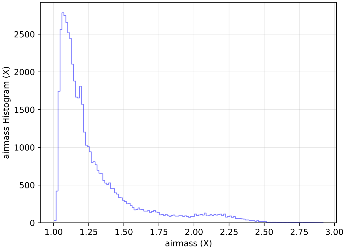
too_elab_r64_d3_ugrizy_v3.4_10yrs Yr 1 r band: airmass Histogram
