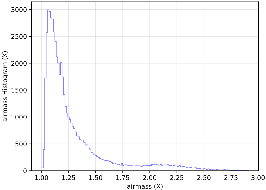
too_elab_r64_d3_ugrizy_v3.4_10yrs Yr 1 i band: airmass Histogram
