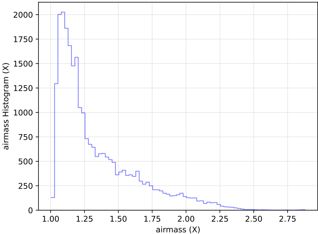
too_elab_r64_d3_ugrizy_v3.4_10yrs Yr 1 g band: airmass Histogram
