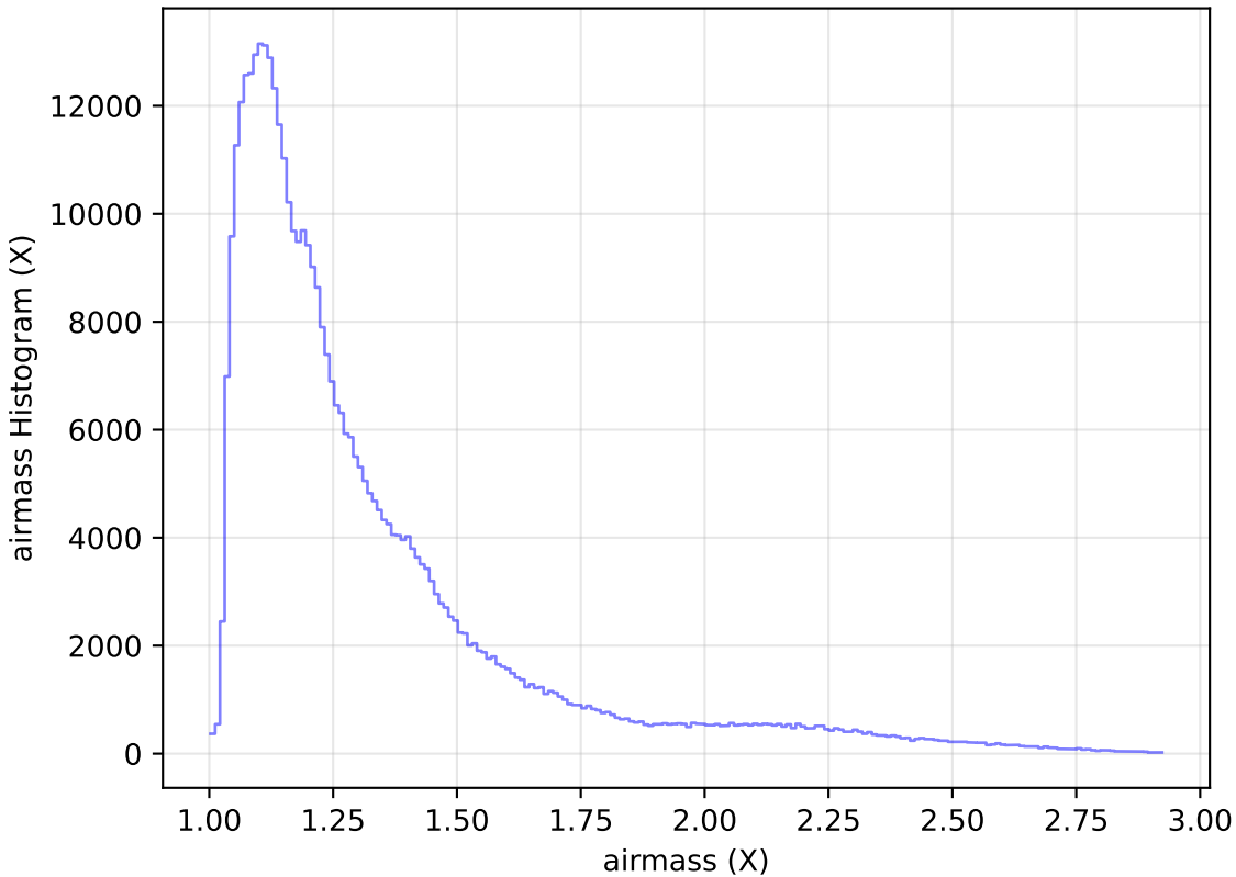
too_elab_r64_d3_ugrizy_v3.4_10yrs WFD z band: airmass Histogram
