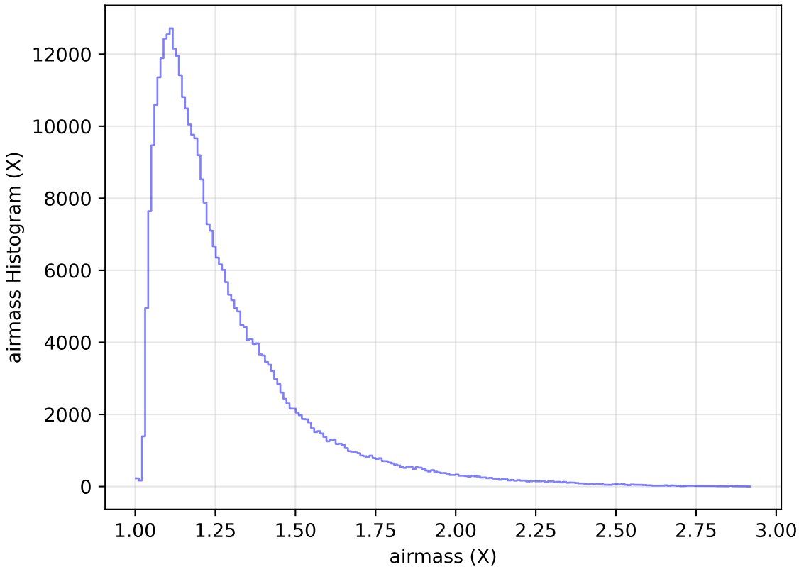
too_elab_r64_d3_ugrizy_v3.4_10yrs WFD y band: airmass Histogram
