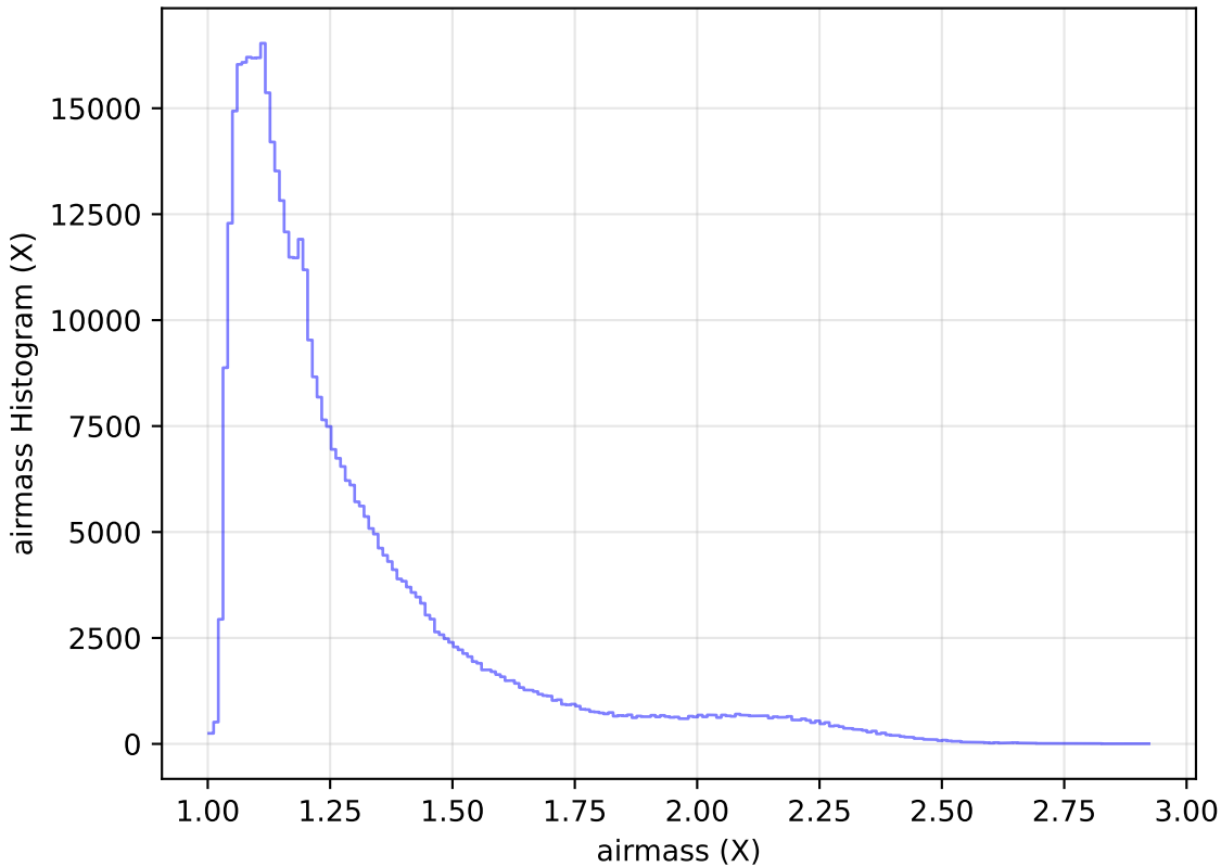
too_elab_r64_d3_ugrizy_v3.4_10yrs WFD r band: airmass Histogram
