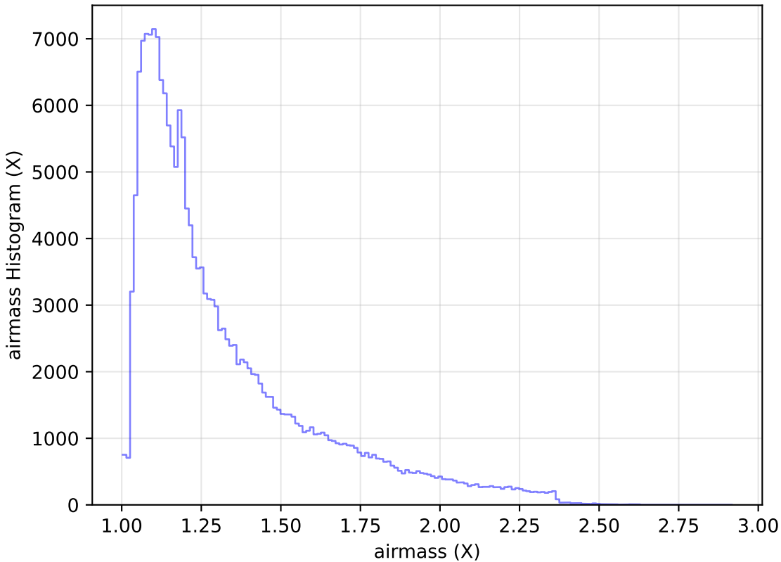
too_elab_r64_d3_ugrizy_v3.4_10yrs WFD g band: airmass Histogram
