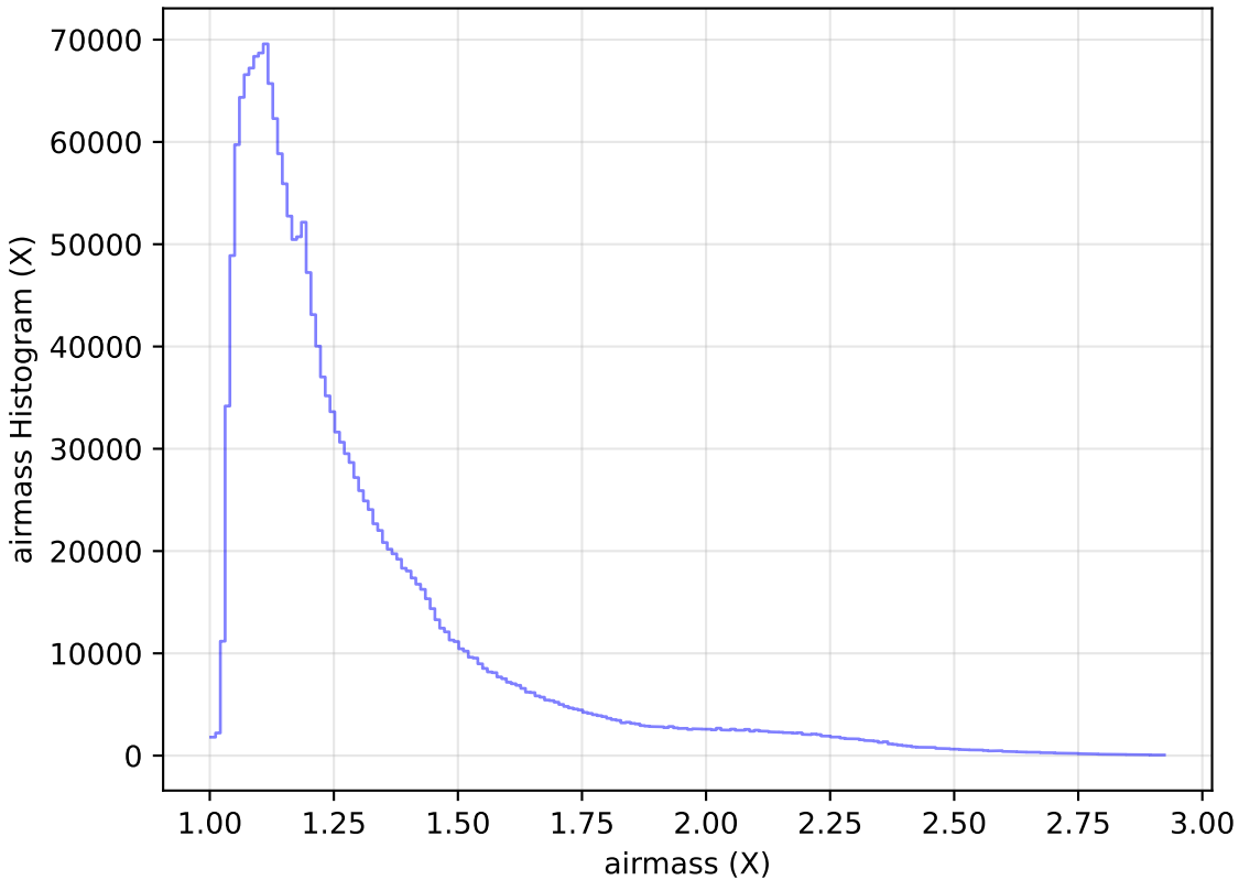
too_elab_r64_d3_ugrizy_v3.4_10yrs WFD all bands: airmass Histogram
