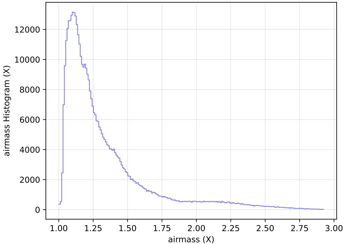
too_elab_r64_d3_ugrizy_v3.4_10yrs All sky z band: airmass Histogram
