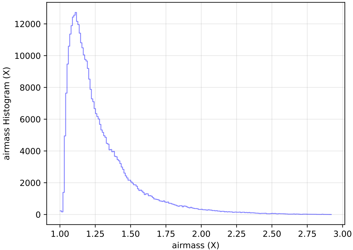
too_elab_r64_d3_ugrizy_v3.4_10yrs All sky y band: airmass Histogram
