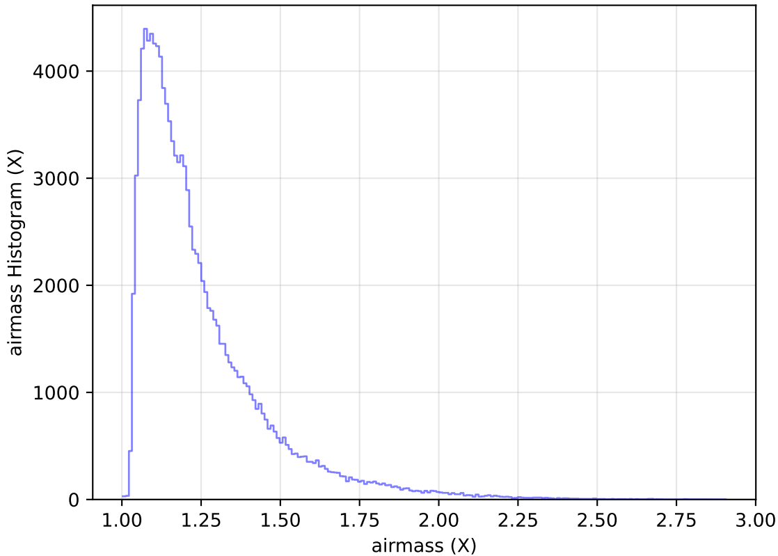
too_elab_r64_d3_ugrizy_v3.4_10yrs All sky u band: airmass Histogram
