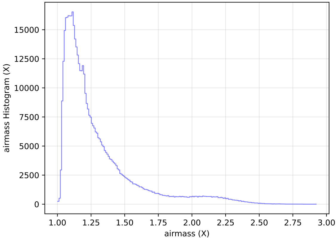
too_elab_r64_d3_ugrizy_v3.4_10yrs All sky r band: airmass Histogram
