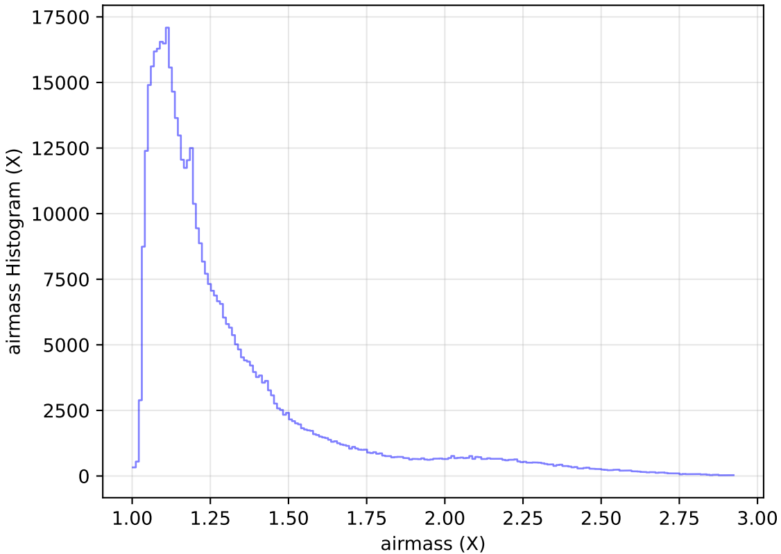
too_elab_r64_d3_ugrizy_v3.4_10yrs All sky i band: airmass Histogram
